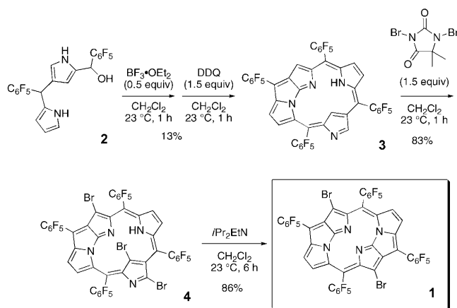
Scheme 1. Preparation of doubly N-fused porphyrin. DDQ = 2,3-dichloro-5,6-dicyanobenzoquinone.
